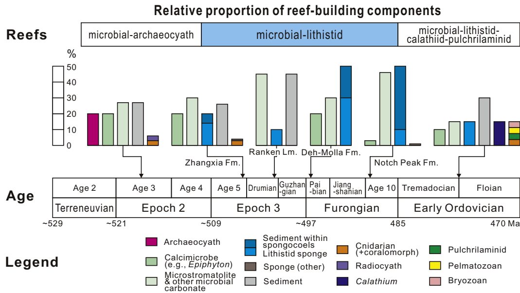
Fig. 3. Relative proportions of main reef components during the Cambrian and Early Ordovician. Early Cambrian microbial-archaeocyath reefs from Gandin and Debrenne (2010), Early Ordovician microbial-lithistid-calathiid reefs from Hong et al. (2015), Li et al. (2015) and references therein. Proportions of mid-late Cambrian reef-building components based on examples in Table 1.
