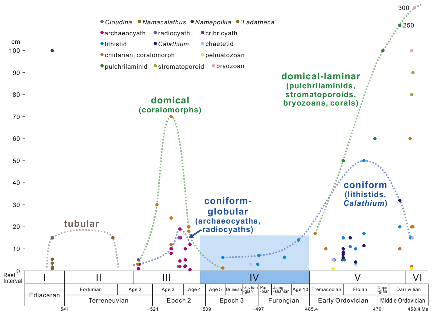
Fig. 8. Size patterns of late Ediacaran to Middle Ordovician reef-building skeletal organisms based on examples in Supplementary Table 1. Three major morphotypes are emphasized: tubular, coniform-globular, domical-laminar. Tubular Cloudina and “ Ladatheca ” occur in the late Ediacaran and early Cambrian, respectively. Coniform sponges (archaeocyaths, lithistids, Calathium ), augmented by globular radiocyaths, are locally conspicuous in Cambrian and Early Ordovician reefs. Domical-laminar forms are represented by coralomorphs in Cambrian Age 2–4, and by pulchrlaminids, stromatoporoids, bryozoans and corals in the Ordovician. These data suggest peaks in skeletal reef-builder size in Reef Interval III and in Reef Intervals V and VI, with smaller skeletons during Reef Interval IV. Reef intervals: I, microbial- Cloudina ; II, microbial-“ Ladatheca ”; III, microbial-archaeocyath; IV, microbial-lithistid; V, microbial-lithistid-calathiid-pulchrlaminid; VI, stromatoporoid-bryozoan-tabulate-receptaculitid-microbial.
