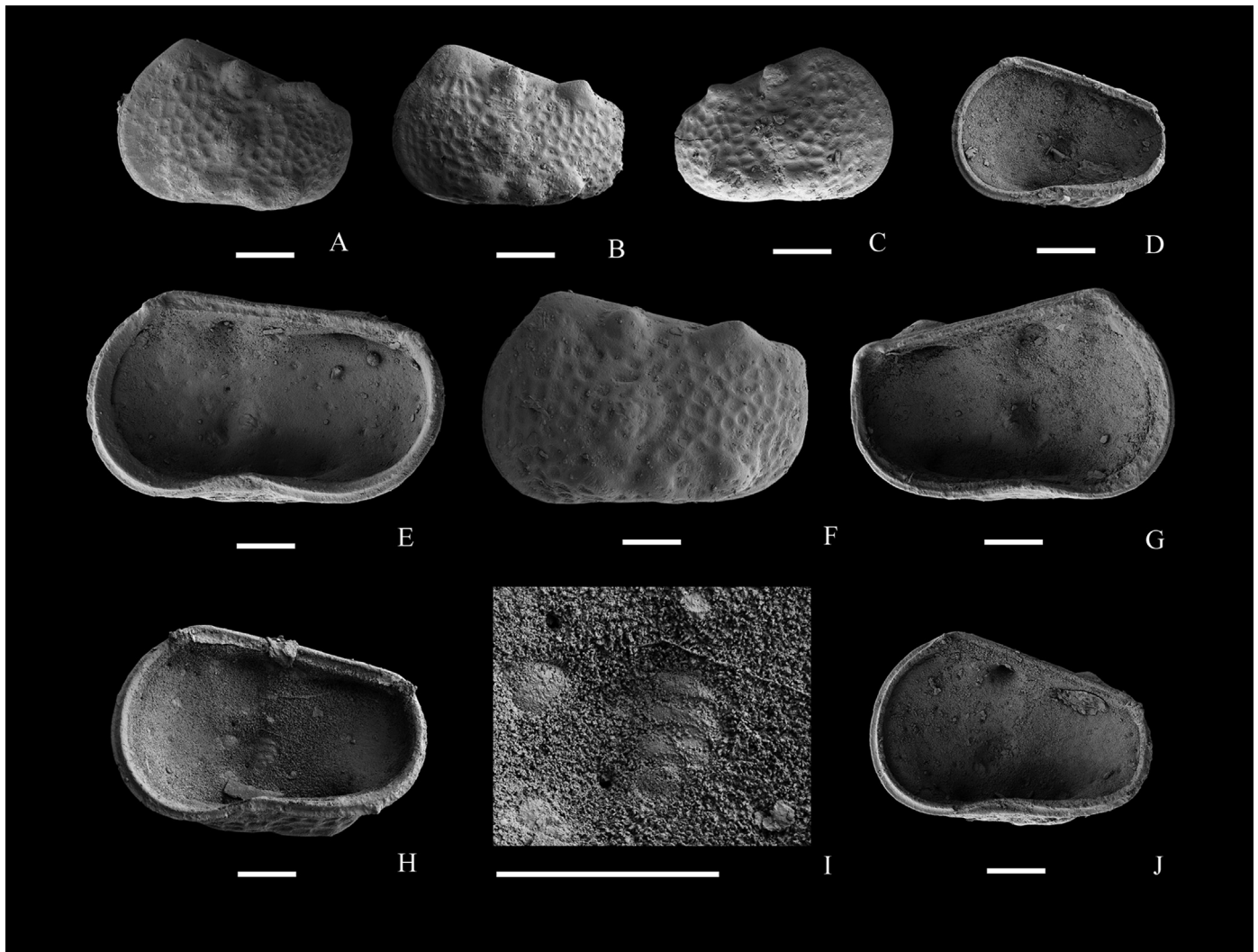
Fig. 12. A–J. Vlakomia jilinensis Gou, 1983; A, left view of juvenile valve (A-3? instar), NIGP 168709, sample 17-TFS-3; B, left view of juvenile valve (A-3? instar), NIGP 168710, sample 17-TFS-2; C, lateral view of juvenile right valve (A-3? instar), NIGP 168711, sample 17-TFS-3; D, internal view of valve (A-3? instar), NIGP 168711, sample 17-TFS-3; E, internal view of male valve (adult), NIGP 68181 (Gou, 1983); F, lateral view of left female valve (adult), NIGP 68182 (Gou, 1983); G, idem, internal view; H, internal view of female valve (adult), NIGP 168712, sample 17-TFS-2; I, idem, muscle scar pattern; J, internal view of juvenile valve (A-2 instar), NIGP 168708, sample 17-TFS-3. Scale bar is 100 \mu m.
