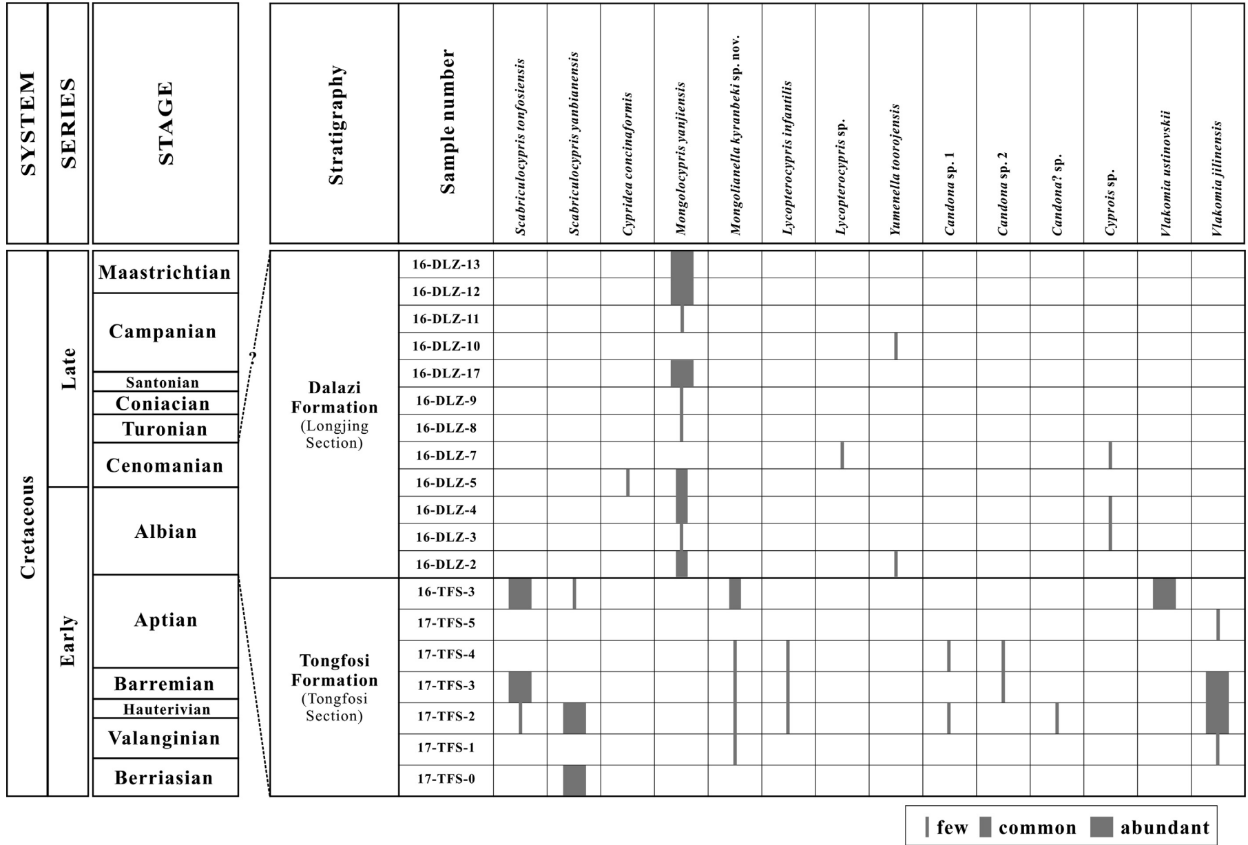
Fig. 3. Stratigraphic distribution and occurrence of ostracod species in the Tongfosi and Dalazi formations of the Yanji Basin.
