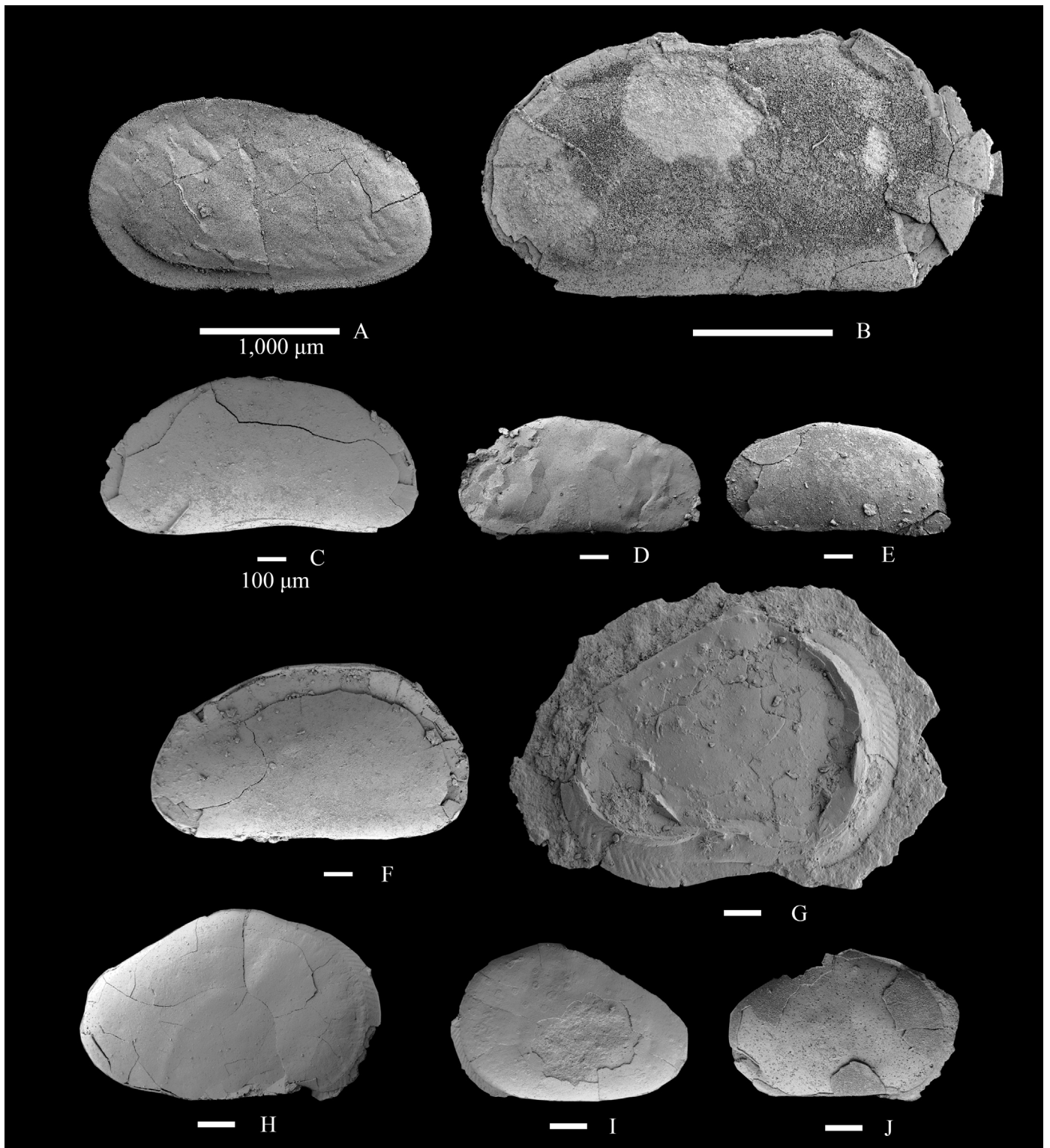
Fig. 9. A–B. Yumenella toorojensis (Khand, 1977); A, left view of presumed male valve, NIGP 168676, sample 16-DLZ-2; B, right view of presumed male carapace, NIGP 168677, sample 16-DLZ-2; C. Candona sp. 1; left view of valve, NIGP 168678, sample 17-TFS-2; D–E. Candona sp. 2; D, right view of valve, NIGP 168679, sample 17-TFS-4; E, right view of valve, NIGP 168680, sample 17-TFS-3; F. Candona ? sp.; left view of valve, NIGP 168681, sample 17-TFS-2; G–J. Cyprois sp.; G, right view of presumed female valve (adult), NIGP 68177; H, right view of valve (juvenile), NIGP 168682, sample 16-DLZ-4; I, left view of valve (juvenile), NIGP 168683, sample 16-DLZ-7; J, right view of valve (juvenile), NIGP 168684, sample 16-DLZ-7.
