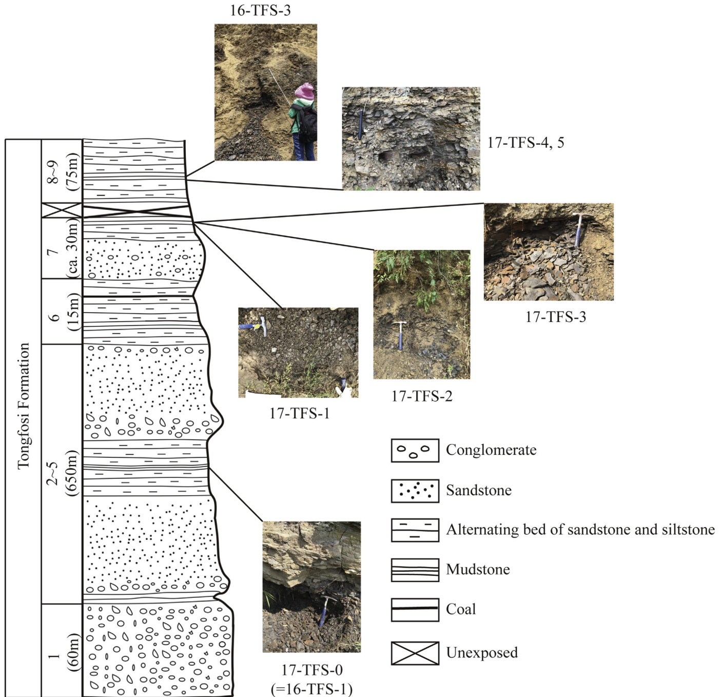
Fig. 2. Lithostratigraphic log of the Tongfosi Formation from the Tongfosi section based on the outcrop description of Zhou et al. (1980) and ostracod sample positions (17-TFS-0 (16-TFS-1): N 42° 53' 40" E 129° 14' 07"; 17-TFS-1: N 42° 53' 49" E 129° 14' 51"; 17-TFS-2: N 42° 53' 37" E 129° 14' 53"; 17-TFS-3: N 42° 53' 37" E 129° 14' 34"; 17-TFS-4, 5: N 42° 53' 30" E 129° 14' 42"; 16-TFS-3: N 42° 53' 33" E 129° 15' 16").
