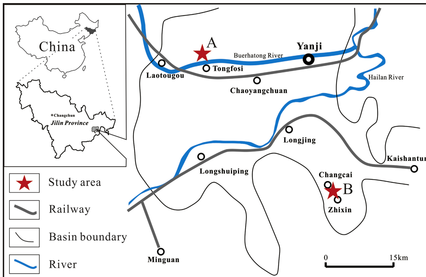
Fig. 1. Location map of the Tongfosi and Dalazi sections (modified from Qiao et al., 2003), A = Tongfosi Section; B = Dalazi Section.
