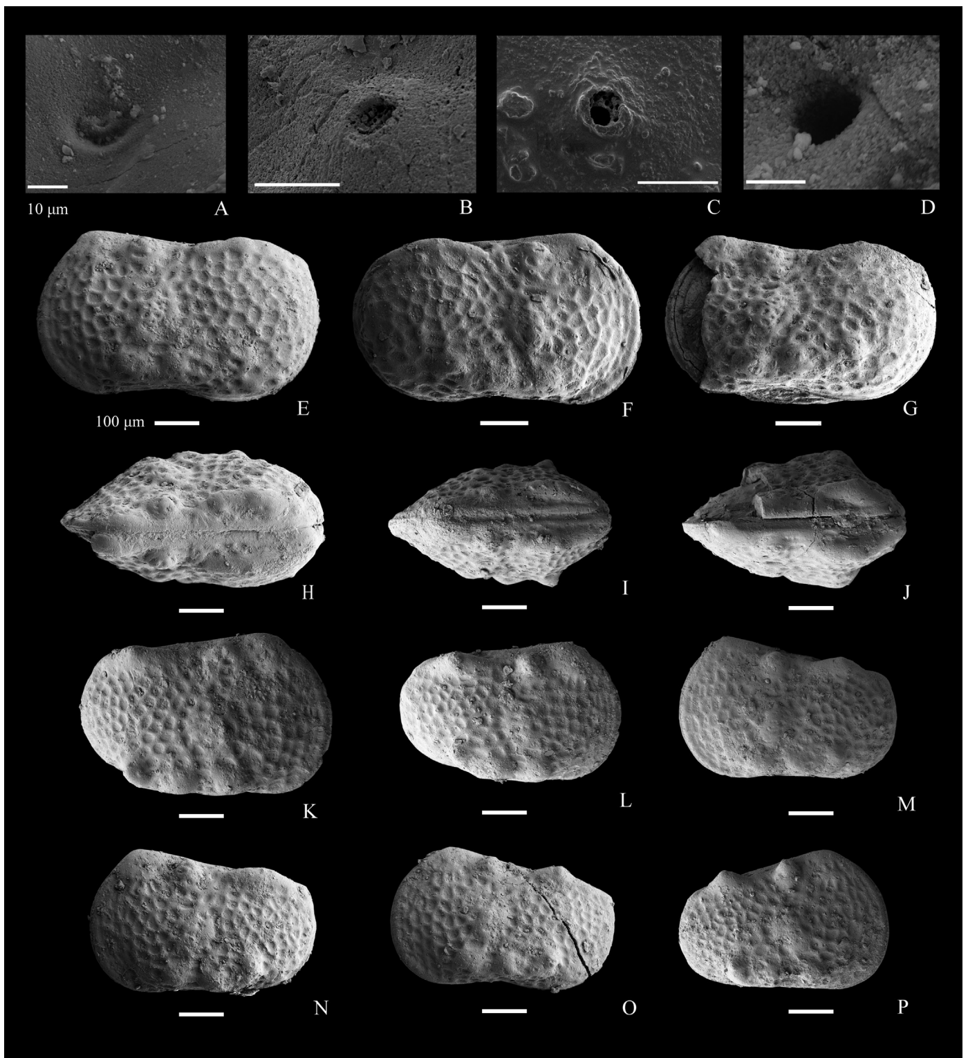
Fig. 11. A–D. Normal pores of Vlakomia ustinovskii Gramm, 1966; A, large normal pore with lip, B, sieve pore, C, sieve pore with sieve plate and central pore, D, canal of pore, inner side view; E–P. Vlakomia jilinensis Gou, 1983; E, left view of male valve (adult), NIGP 168700, sample 17-TFS-3; F, right view of male valve (adult), NIGP 68181 (Gou, 1983); G, left view of male carapace (adult), NIGP 68178 (Gou, 1983); H, idem, dorsal view, anterior end to the left; I, dorsal view of male carapace (A-1 instar), anterior end to the left, NIGP 168701, sample 17-TFS-3; J, dorsal view of female carapace (A-1 instar), anterior end to the left, NIGP 168702, sample 17-TFS-2; K, right view of female valve (adult), NIGP 168703, sample 17-TFS-2; L, right view of female valve (A-1 instar), NIGP 168704, sample 17-TFS-3; M, left view of female valve (A-1 instar), NIGP 168705, sample TFS-3; N, left view of female valve (A-1 instar), NIGP 168706, sample 17-TFS-2; O, left view of female valve (A-1 instar), NIGP 168707, sample 17-TFS-3; P, right view of juvenile valve (A-2 instar), NIGP 168708, sample 17-TFS-3.
