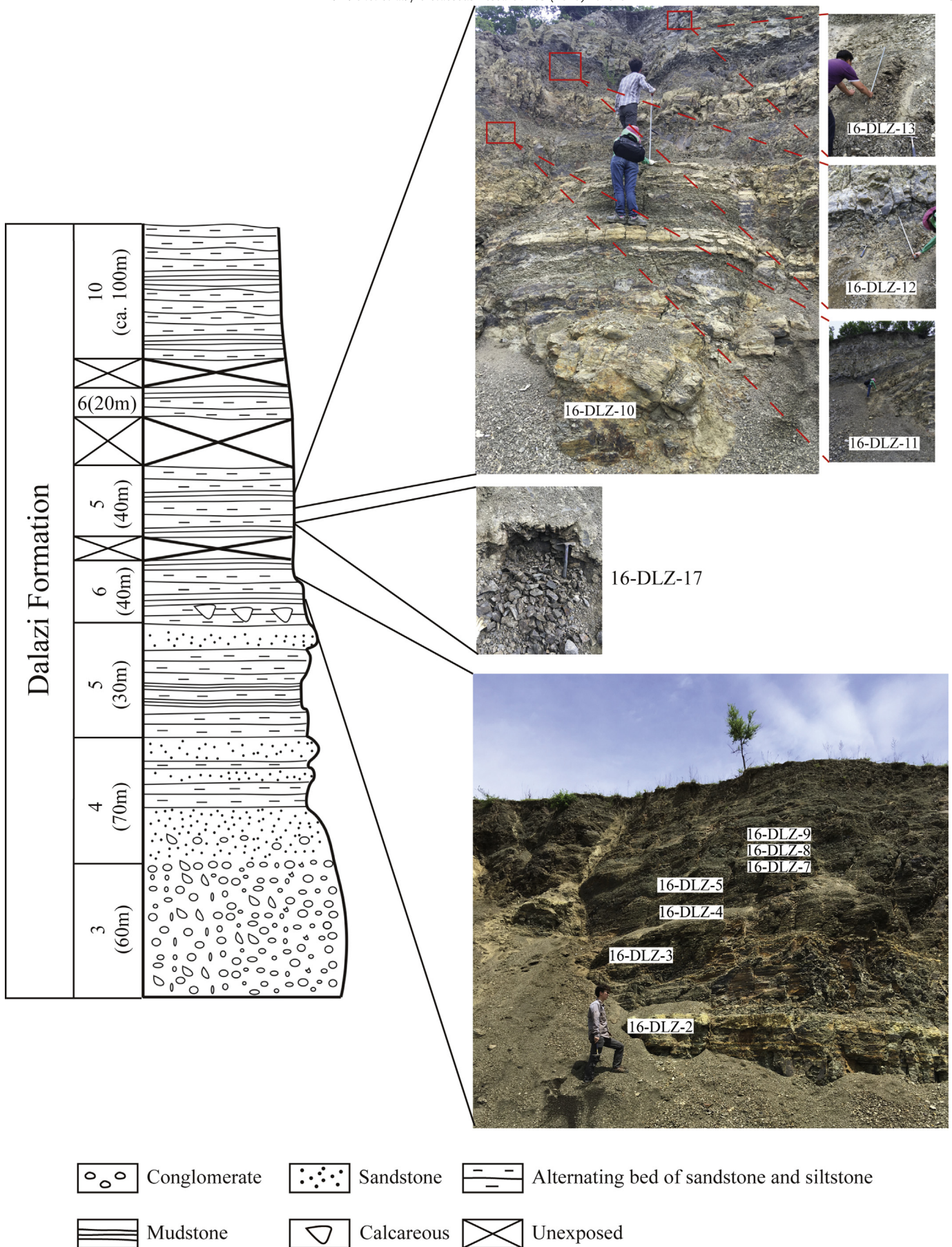
Fig. 4. Lithostratigraphic log of the Dalazi Formation from the Dalazi section based on the outcrop description of Zhou et al. (1980) and ostracod sample positions (16-DLZ-2, 3, 4, 5, 7, 8, 9: N 42° 39' 58" E 129° 32' 57"; 16-DLZ-17: N 42° 39' 53" E 129° 33' 06"; 16-DLZ-10, 11, 12, 13: N 42° 39' 24" E 129° 33' 35").
