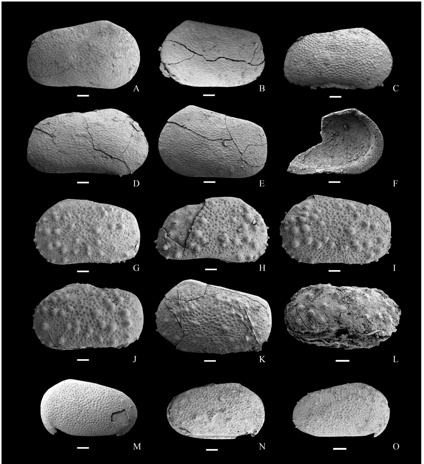
Fig. 5. A–F. Scabriculocypris tonfosiensis Gou, 1983; A, right view of valve, NIGP 68168 (Gou, 1983 holotype); B, left view of valve, NIGP 168645, sample 17-TFS-2; C, right view of valve, NIGP 168646, sample 17-TFS-3; D, right view of valve, NIGP 168647, sample 17-TFS-3; E, left view of valve, NIGP 168648, sample 17-TFS-3; F, internal view of partial anterior valve, NIGP 168649, sample 17-TFS-3; G–L. Scabriculocypris yanbianensis (Gou, 1983); G, left view of valve, NIGP 68169 (Gou, 1983 holotype); H, right view of valve, NIGP 68170 (Gou, 1983 paratype); I, left view of valve, NIGP 68171 (Gou, 1983 paratype); J, left view of valve, left view of valve, NIGP 68172 (Gou, 1983 paratype); K, left view of valve, NIGP 168650, sample 17-TFS-2; L, left view of core (no shell), NIGP 168651, sample 17-TFS-0; M–O. Cypridea concinaformis Su, 1974; M, left view of valve, NIGP 168652, sample 16-DLZ-5; N, right view of carapace, NIGP 68163 (Gou, 1983); O, right view of valve, NIGP 68164 (Gou, 1983). Scale bar is 100 \mu m.
