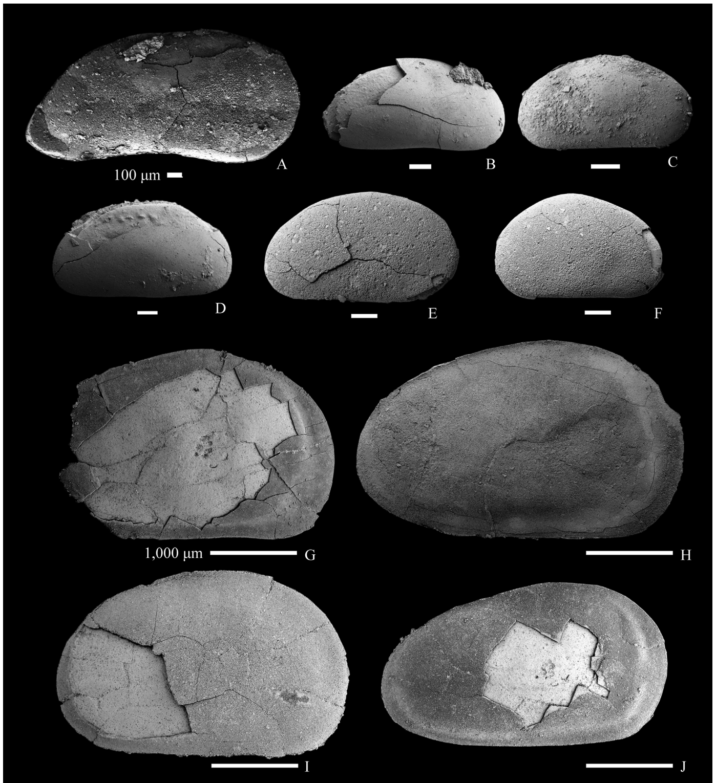
Fig. 8. A. Mongolianella kyranbeki sp. nov., right view of valve, NIGP 168666, sample 17-TFS-2; B–D. Lycopteroocypris infantilis ; B, lateral view of right valve, NIGP 168667, sample, C, right view of valve, NIGP 168668, sample 17-TFS-3; D, left view of valve, NIGP 168669, sample 17-TFS-4; E–F. Lycopteroocypris sp.; E, right view of valve, NIGP 168670, sample 16-DLZ-7; F, left view of valve, NIGP 168671, sample 16-DLZ-7; G–J. Yumenella toorojensis (Khand, 1977); G, right view of presumed female valve, NIGP 168672, sample 16-DLZ-2; H, right view of presumed male valve, NIGP 168673, sample 16-DLZ-2; I, right view of female valve, NIGP 168674, sample 16-DLZ-2; J, right view of presumed male valve, NIGP 168675, sample 16-DLZ-2.
