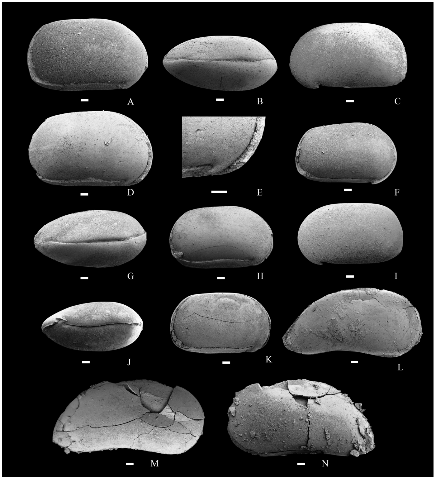
Fig. 7. A–K. Mongolocypis yanjiensis Gou, 1983; A, right view of carapace (adult), NIGP 168653, sample 16-DLZ-12; B, dorsal view of carapace (adult), anterior end to the left, NIGP 168654, sample 16-DLZ-13; C, left view of carapace (adult), NIGP 168655, sample 16-DLZ-12; D, right view of carapace, NIGP 168656, sample 16-DLZ-13; E, idem, right lateral of anteroventral region, rostrum and alveolus; F, right view of carapace (A1 instar), NIGP 168657, sample 16-DLZ-17; G, dorsal view of carapace (adult), anterior end to the left, NIGP 168658, sample 17-DLZ-17; H, right view of carapace (A-1 instar), NIGP 168659, sample 16-DLZ-17; I, left view of carapace (A-1 instar), NIGP 168660, sample 16-DLZ-17; J, ventral view of carapace (A-1 instar), anterior end to the left, NIGP 168661, sample 16-DLZ-17; K, right view of carapace (A-1 instar), NIGP 168662, sample 16-DLZ-17; L–N. Mongolianella kyranbeki sp. nov.; L, lateral view of right valve, NIGP 168663 (holotype), sample 16-TFS-3; M, lateral view of right valve, NIGP 168664, sample 17-TFS-2; N, lateral view of left valve, NIGP 168665, sample 17-TFS-2. Scale bar is 100 \mu m.
