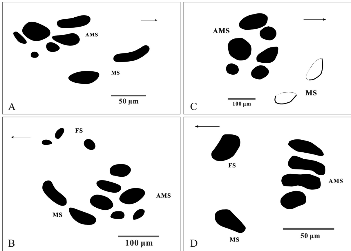
Fig. 6. Line drawing of muscle scars: A, Scabriculocypris tonfosiensis Gou, 1983; B, Mongolianella kyranbeki sp. nov.; C, Yumenella toorojensis (Khand, 1977); D, Vlakomia jilinensis Gou, 1983.
