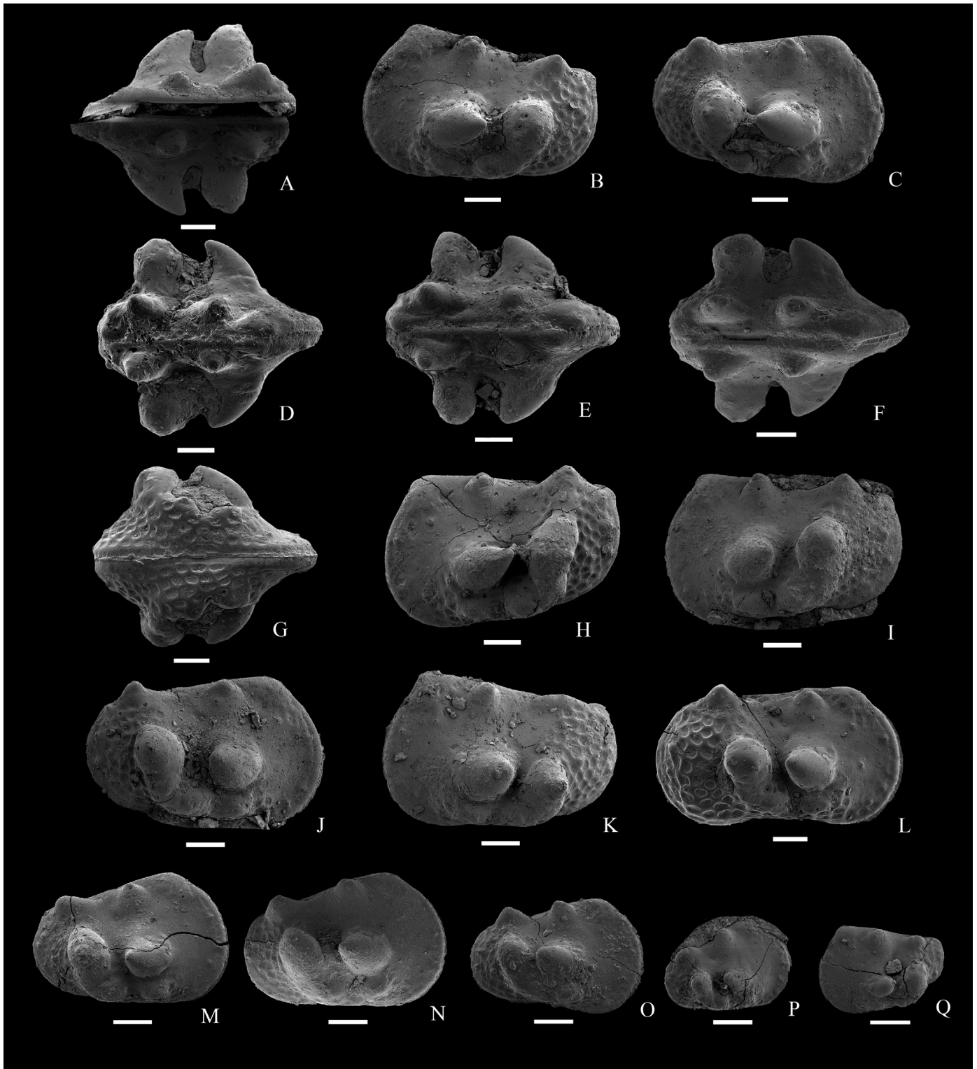
Fig. 10. A–Q, Vlakomia ustinovskii Gramin, 1966; A, dorsal view of female carapace, NIGP 168685, sample 16-TFS-3; B, lateral view of female left valve, NIGP 168685, sample 16-TFS-3; C, lateral view of female right valve, NIGP 168685, sample 16-TFS-3; D, dorsal view of female carapace, NIGP 168686, sample 16-TFS-3; E, dorsal view of female carapace, NIGP 168687, sample 16-TFS-3; F, dorsal view of female carapace (adult), NIGP 168688, sample 16-TFS-3; G, ventral view of female carapace (adult), NIGP 168689, sample 16-TFS-3; H, lateral view of female left valve (adult), NIGP 168690, sample 16-TFS-3; I, lateral view of female left valve (adult), NIGP 168691, sample 16-TFS-3; J, lateral view of female right valve (adult), NIGP 168692, sample 16-TFS-3; K, lateral view of female left valve (adult), NIGP 168693, sample 16-TFS-3; L, lateral view of male right valve (adult), NIGP 168694, sample 16-TFS-3; M, lateral view of right valve (A-1 instar), NIGP 168695, sample 16-TFS-3; N, lateral view of right valve (A-1 instar), NIGP 168696, sample 16-TFS-3; O, lateral view of right valve (A-2? instar), NIGP 168697, sample 16-TFS-3; P, lateral view of right valve (A-3? instar), NIGP 168698, sample 16-TFS-3; Q, lateral view of left valve (A-3? instar), NIGP 168699, sample 16-TFS-3. Scale bar is 100 \mu m.
