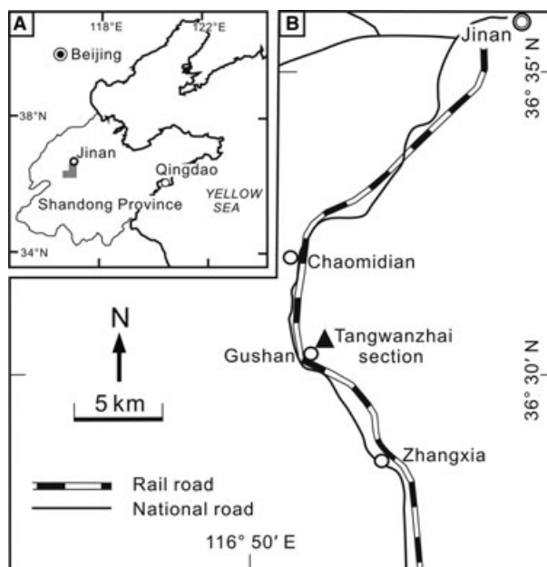
FIG. 1. Location maps. A, index map displaying the approximate location of the study area (shaded) in Shandong Province, China. B, the Tangwangzhai section (solid triangle), from which the material for study was collected, is located about 25 km south-west of Jinan, capital of the Shandong Province.
