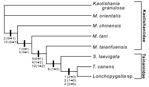
FIG. 8. Cladogram showing the relationship between the Kaolishaniidae and the Tsinaniidae. Only unambiguous characters are shown at each node with the state change indicated. See text for explanation.
